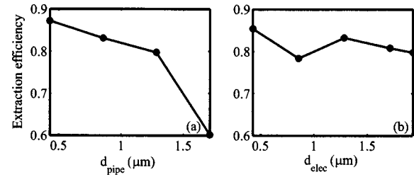
FIG. 7. (a) The extraction efficiency at the resonant frequency and at the cavity center in the QW [Fig. 1(b)] as a function of d_{\text{pipe}} . (b) The extraction efficiency at the resonant frequency and at the cavity center in the QW as a function of d_{\text{elec}} . All other parameters are as in the reference structure [Fig. 1(b)].
