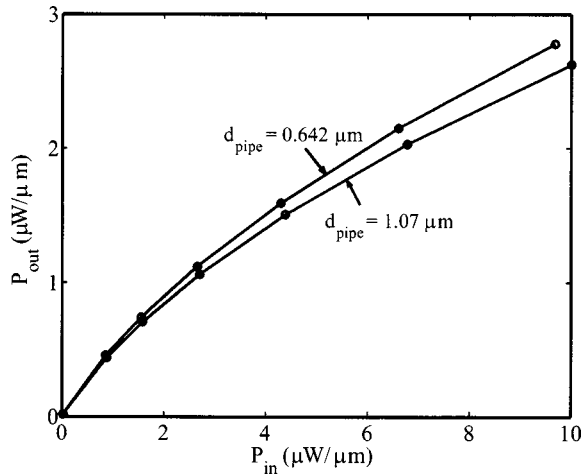
FIG. 8. The total light output power per unit length extracted from the device as a function of the input electrical power per unit length for two different values of d_{pipe} . The doping configuration is p - i - n . All other parameters are as in the reference structure [Fig. 1(b)].
