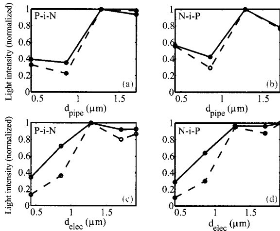
FIG. 6. (a) and (b) The light power generated in the QW at the cavity center [Fig. 1(b)] and at the resonance wavelength of \sim 850 nm as a function of d_{\text{pipe}} . (c) and (d) The light power generated in the QW at the cavity center and at the resonance wavelength as a function of d_{\text{elec}} . In (a) and (c) [(b) and (d)], the doping configuration is p-i-n ( n-i-p ). We also show with a dashed line the product of the electron and hole densities at the cavity center and of the enhancement factor at the cavity center and at the resonance wavelength. All other parameters are as in the reference structure [Fig. 1(b)]. All quantities are normalized with respect to their maximum value.
