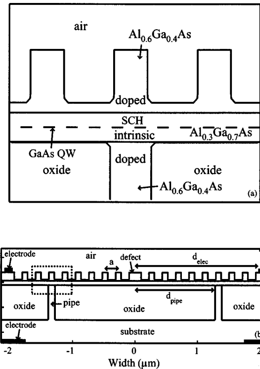
FIG. 1. (a) The p-i-n device structure. The \text{Al}_{0.3}\text{Ga}_{0.7}\text{As} separate-confinement heterostructure (SCH) and the active region, consisting of an 80-Å GaAs QW, are undoped. The SCH is surrounded by \text{Al}_{0.6}\text{Ga}_{0.4}\text{As} doped to a density of 10^{18} \text{ cm}^{-3} on both the p side and the n side. (b) The device geometry. The period of the grating is a=0.214 \mu\text{m} . The reference device structure is characterized by d_{\text{pipe}}=1.284 \mu\text{m} and d_{\text{elec}}=1.926 \mu\text{m} . We also show with dashed lines the device area magnified in (a).
