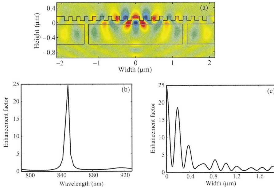
FIG. 2. (a) (Color) The electric-field profile when a dipole is placed in the QW at the center of the cavity defect and emitting at the resonant frequency of the cavity mode. (b) The calculated spontaneous emission enhancement factor as a function of wavelength for a dipole placed in the QW at the center of the cavity defect. (c) The calculated enhancement factor at the cavity resonant frequency as a function of emitter position in the QW.
