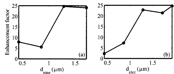
FIG. 5. (a) The spontaneous emission enhancement factor at the resonant frequency and at the cavity center in the QW [Fig. 1(b)] as a function of d_{\text{pipe}} . (b) The spontaneous emission enhancement factor at the resonant frequency and at the cavity center in the QW as a function of d_{\text{elec}} . All other parameters are as in the reference structure [Fig. 1(b)].
