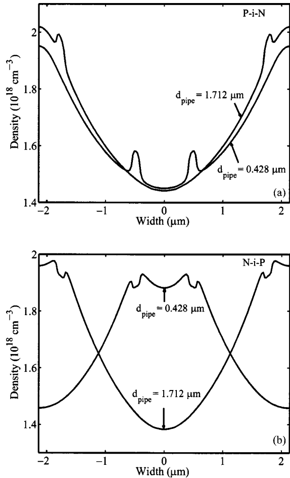
FIG. 3. (a) The electron-density profile in the QW for the p-i-n configuration. (b) The electron-density profile in the QW for the n-i-p configuration. Results are shown for d_{\text{pipe}}=0.428 \mu\text{m} and d_{\text{pipe}}=1.712 \mu\text{m} . All other parameters are as in the reference structure [Fig. 1(b)].
