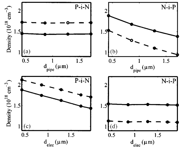
FIG. 4. (a) and (b) The electron and hole densities in the QW at the cavity center [Fig. 1(b)] as a function of d_{\text{pipe}} . (c) and (d) The electron and hole densities in the QW at the cavity center as a function of d_{\text{elec}} . In (a) and (c) [(b) and (d)], the doping configuration is p-i-n ( n-i-p ). Hole densities are shown with a dashed line. All other parameters are as in the reference structure [Fig. 1(b)].
