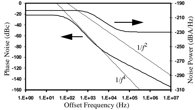
Fig. 6. Phase noise generated by a combination of Lorentzian and white noise sources
