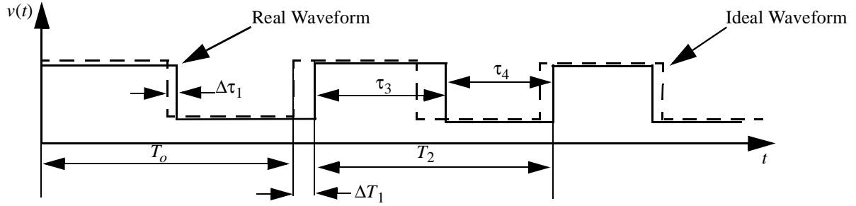
Fig. 1. Real and ideal waveforms for a rectangular oscillatory signal with parameter definitions.
