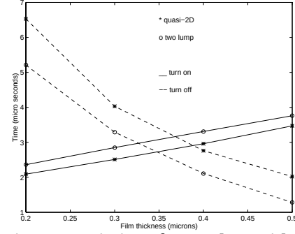
Fig. 12: Variation of t_{on} and t_{off} with film thickness, h , in Type II switch
