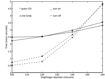
Fig. 13: Variation of t_{on} and t_{off} with diaphragm diameter, W_d , in Type I switch
