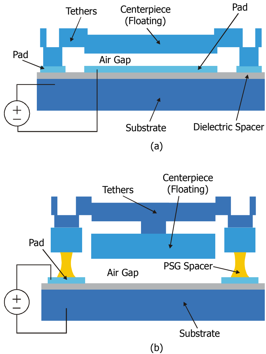
Figure 6. Cross sections of folded capacitor structures. (a) Structure using the nitride layer as the dielectric spacer. Centerpiece and tethers are made from POLY1. (b) PSG forms the dielectric spacer after a controlled HF etch. The tethers, made from POLY2, are shielded from the substrate electrode by the centerpiece, thus reducing parasitics.
