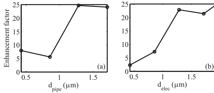
Figure 5. (a) The spontaneous emission enhancement factor at the resonant frequency and at the cavity center in the QW (Fig. 1b) as a function of d_{\text{pipe}} . (b) The spontaneous emission enhancement factor at the resonant frequency and at the cavity center in the QW as a function of d_{\text{elec}} . All other parameters are as in the reference structure (Fig. 1b).
